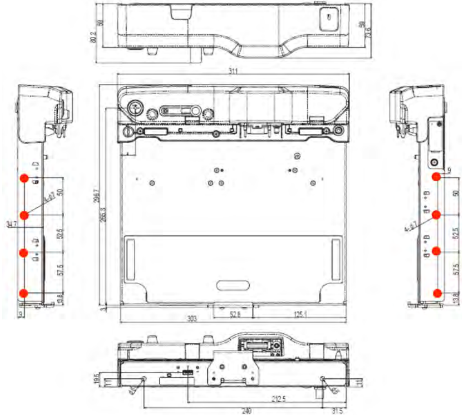
Figure 2 - Docking Station Dimensions (In millimeters)
